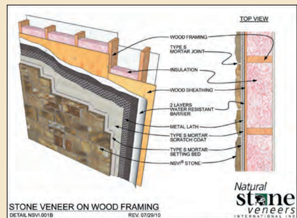
Stone Veneer on Wood Framing
